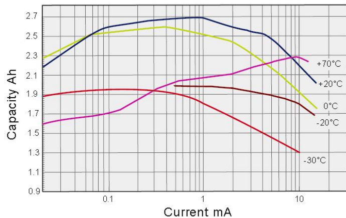
Temperature characteristics
